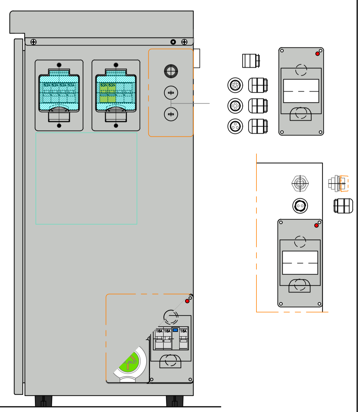
SIDE VIEW
