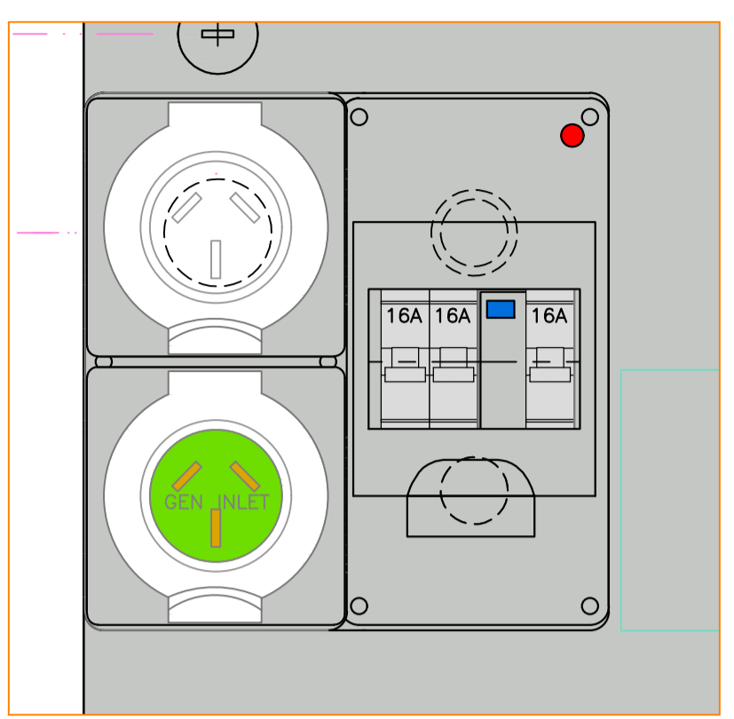
CONNECTIONS DETAILS SCALE 1:2.5
