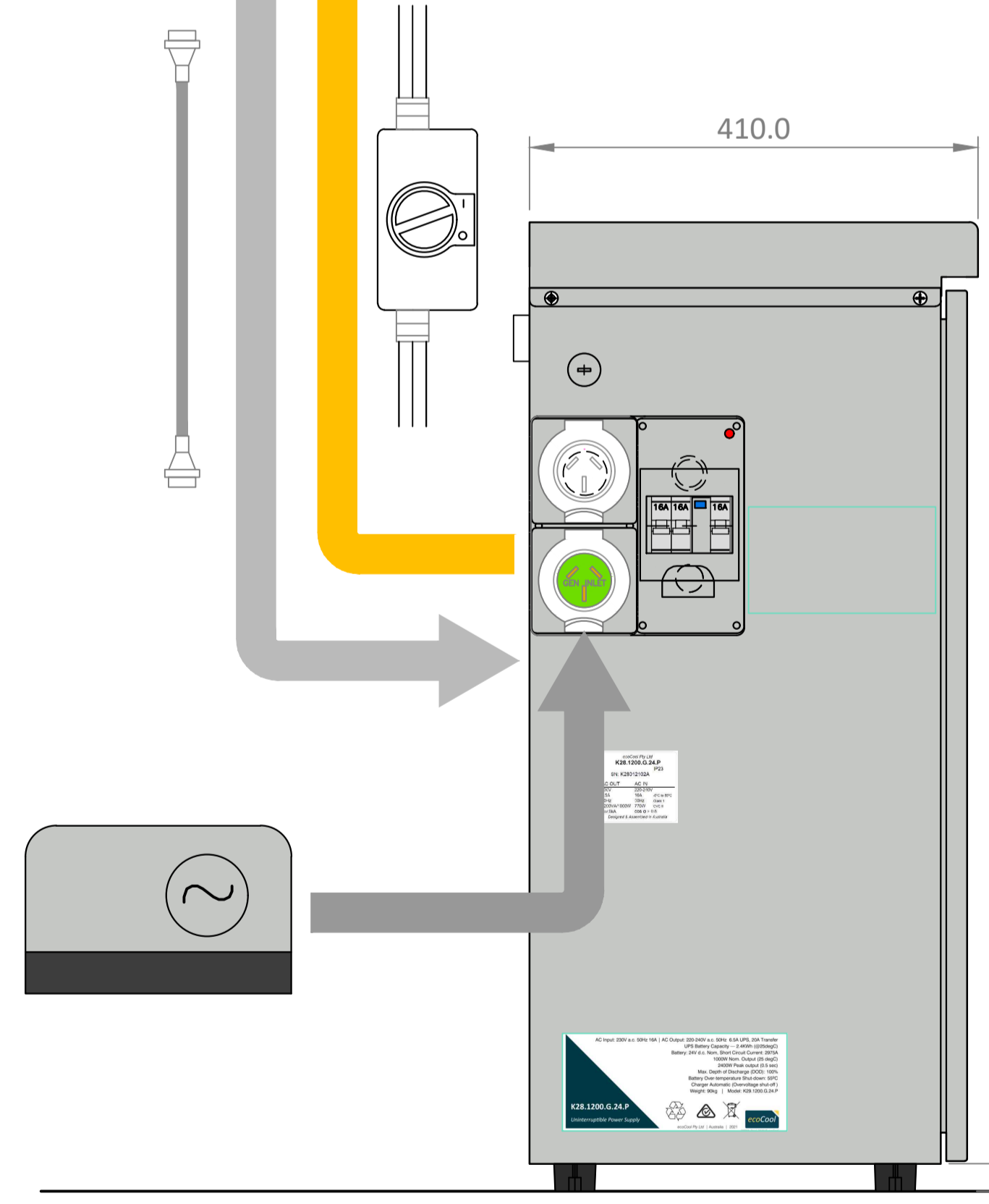
SIDE VIEW
